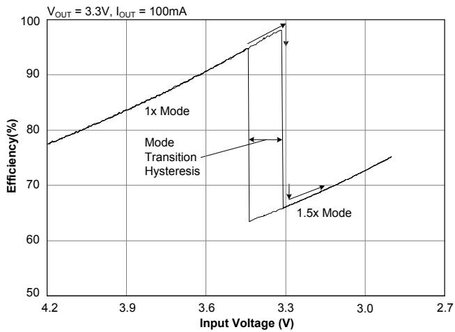
Efficiency — 100mA
