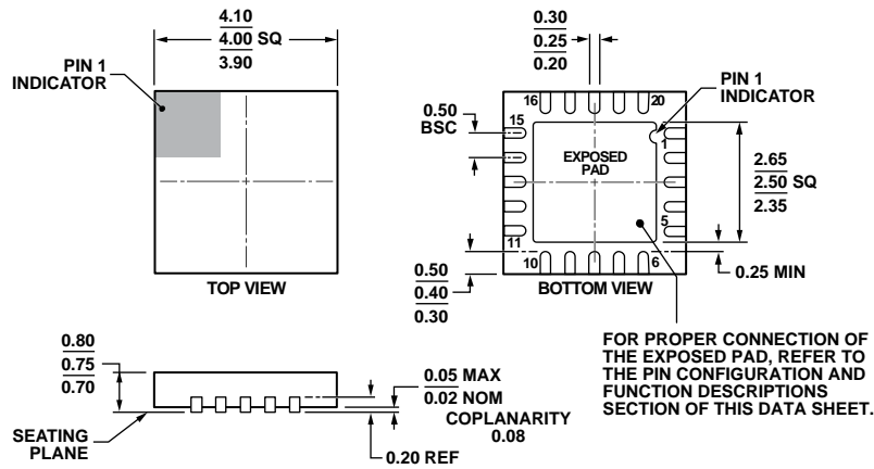
Figure 42. 20 Lead Lead Frame Chip Scale Package [LFCSP_WQ] 4 mm x 4 mm Body, Very Very Thin Quad (CP-20-10) Dimensions shown in millimeters
